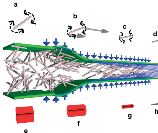
Fig. 15 Illustration for the use of hydrodynamic-focusing microfluidics to produce filaments from a dispersion of cellulose nanofibrils; (reproduced from) reprinted with permission from Macmillan Publishers Ltd. [Nature] (Håkansson et al. 17 ), copyright (2014).
