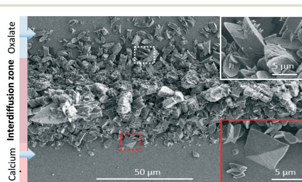
Fig. 2 SEM image of precipitated crystals obtained in the microfluidic device from oxalate and calcium solutions at the dynamic interface. The white inset shows a zoom of the upper part of the precipitate containing twinned crystals. The red inset shows a zoom of the lower part of the precipitate containing mixed twinned and tapered bipyramid crystals.
