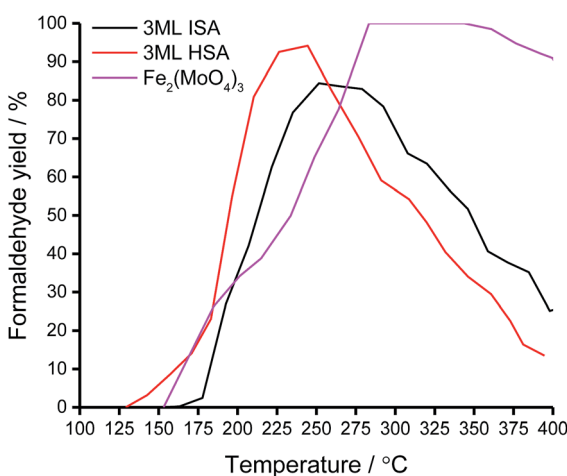
Fig. 8 Formaldehyde yield of the bulk and shell@core iron molybdate catalysts under the TPPFR of methanol.
