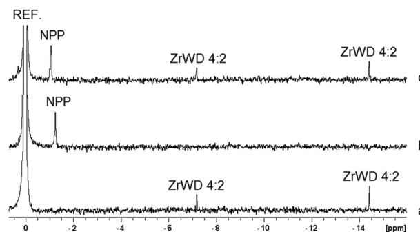
Fig. 6 31 P NMR spectra of (a) 1.0 mM of ZrWD 4 : 2, (b) 5.0 mM NPP and (c) the mixture of 5.0 mM of NPP and 1.0 mM of ZrWD 4 : 2 after adjusting the pD to 6.4 (400 MHz, D 2 O, 293 K, NS = 256, 25% H 3 PO 4 ).
