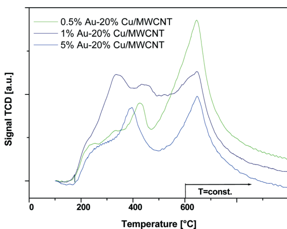
Fig. 9 TPD-NH 3 profile of the bimetallic catalysts 1) 0.5% Au–20% Cu/MWCNT, 2) 1% Au–20% Cu/MWCNT, and 3) 5% Au–20% Cu/MWCNT after calcination in air for 4 h at 180 °C and reduction in a mixture of 5% H 2 –95% Ar at 300 °C.
