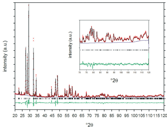
Fig. 5 Graph of the Rietveld refinement on BiYWO 6 . The observed diffractogram is represented by red dots, the calculated diffractogram by a black line, the difference between them ( I_o - I_c ) by a green line, and the background by a blue line.
