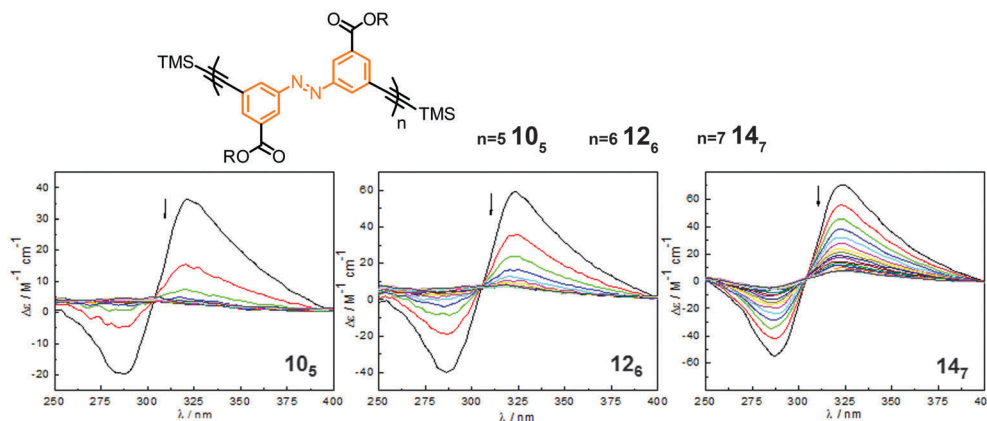
Fig. 14 Photoswitchable oligoazobenzene foldamers 10 5 , 12 6 , and 14 7 ( R = -(\text{CH}_2\text{CH}_2\text{O})_3\text{CH}_3 or -(\text{CH}(\text{S}-\text{CH}_3)\text{CH}_2\text{O})(\text{CH}_2\text{CH}_2\text{O})_3\text{CH}_3 ) and their corresponding CD spectra during the course of irradiation at \lambda_{\text{irr}} = 358 \text{ nm} in \text{CH}_3\text{CN} at 25 °C. 45
