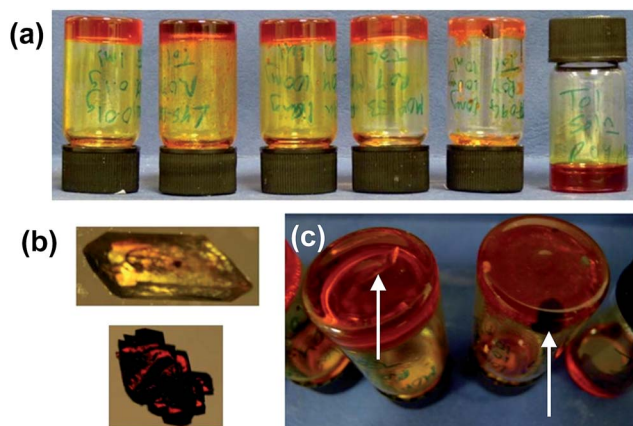
Fig. 2 (a) Crystals of ROY grown from four non-specific control gels and from gels of 2 (left to right: 3 – 6 and 2 ) and a solution phase control experiment. (b) Isolated gel-grown crystals of the Y and R forms. (c) Y-Form crystals growing in a toluene gel of non-specific gelator 6 (left) and R-form crystals growing in toluene gel of 2 , (right; arrows point to individual crystals).
