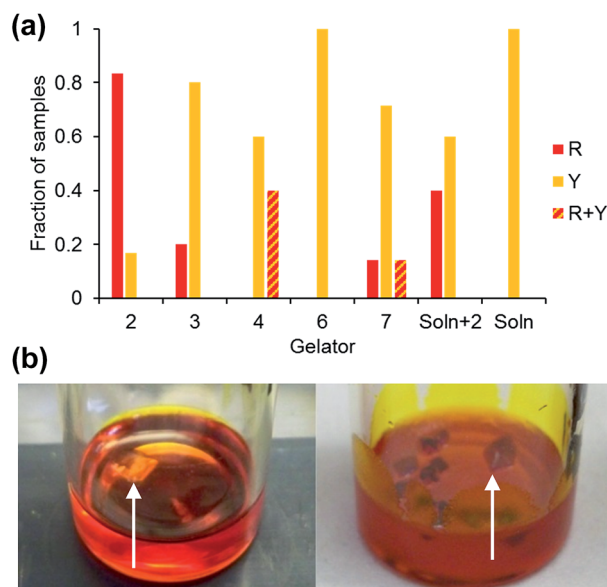
Fig. 3 (a) Collated data comparing the form of ROY obtained from 100 mg mL −1 toluene gels of designer gelator 2 , non-specific gelators 3 , 4 , 6 and 7 , from toluene solution saturated with 2 and from solution. R + Y denotes concomitant crystallisation of both the R and Y crystal forms in the same sample. (b) Crystallization of the Y form of ROY from a toluene gel of control compound 7 and the R form from a toluene gel of 2 (arrows point to individual crystals).
