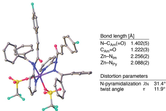
Fig. 6 Crystal structure of (1a)_2/Zn with selected structural parameters. Hydrogen atoms are omitted for clarity. Color code: gray = carbon, blue = nitrogen, red = oxygen, sky blue = fluorine, yellow = sulfur, and purple = zinc.
