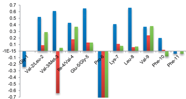
Fig. 6 NMR analysis. Plot of difference between H \alpha chemical shift values in the random coil and the values determined experimentally for G2a (blue) and isomers G1a-1 (red) and G1a-2 (green) in CD 3 OH at 298 K.
