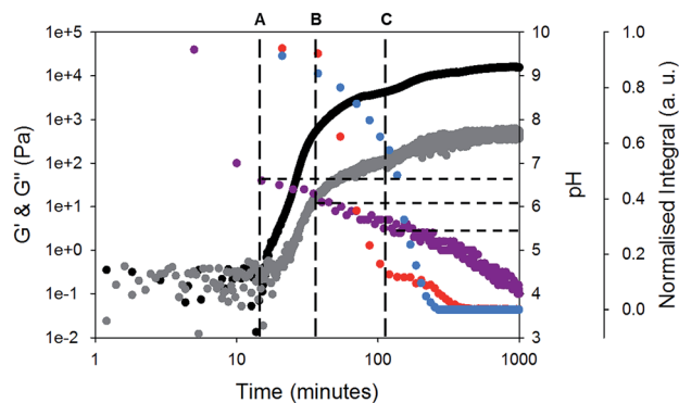
Fig. 3 Monitoring gelation of 1 and 2 over time. The change in intensity of peaks from 1 H NMR spectroscopy during gelation of the CH 3 peak at 1.70 ppm from gelator-1 (blue) and the CH 2 at 3.05 ppm from gelator-2 (red) are compared to change in pH during gelation of 1 and 2 (purple). The change in G' and G'' over time for gel-1,2 is also shown (black data are G' and grey data are G'' ), rheological time sweeps were performed at a strain of 0.5%, 10 \text{ rad s}^{-1} and at 25 \text{ }^\circ\text{C} . For discussion around points A, B, and C, please see main text.
