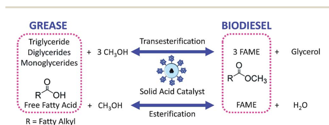
Fig. 6 Esterification of fatty acids and transesterification of triglyceride to produce biodiesel.
