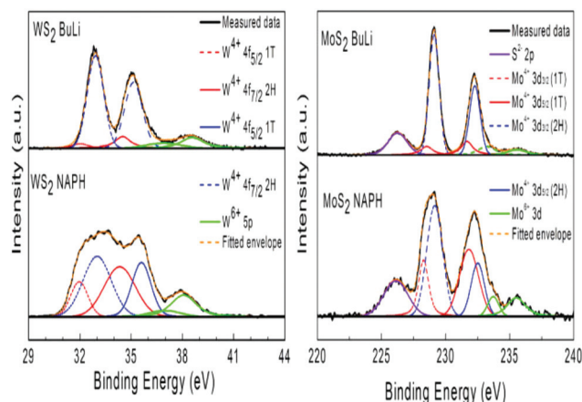
Fig. 3 High-resolution XPS spectra of W 4f in WS 2 and Mo 3d in MoS 2 exfoliated with butyllithium and sodium naphthalenide.
