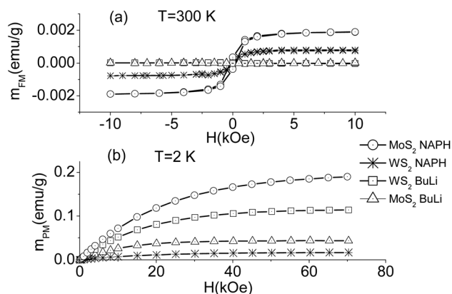
Fig. 6 (a) T = 300 K hysteresis loops for MoS 2 and WS 2 , (b) T = 2 K, magnetization curves for MoS 2 and WS 2 (symbols – measured data, lines – calculation for S = 1 and the corresponding values m_{PM0} , \chi_1 given in Table 2).
