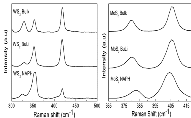
Fig. 2 Raman spectra of exfoliated transition metal dichalcogenides in their bulk state (top), after exfoliation with butyllithium (middle) and after exfoliation with sodium naphthalenide (bottom).
