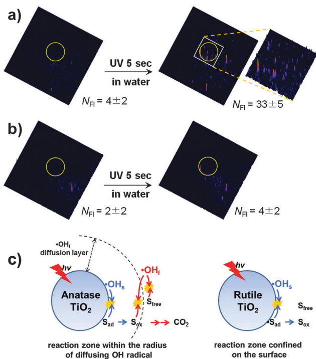
Fig. 2 (a and b) Fluorescence images of free hydroxyl radicals ( \bullet\text{OH}_f ) that migrated through a gap from the UV-illuminated \text{TiO}_2 (a: anatase, b: rutile) to HPF-coated cover glass. The \text{TiO}_2 /water system with silanol-modified HPF (3'-( p -hydroxyphenyl)fluorescein) was compared before (left) and after (right) UV irradiation for 5 s. The diffusion gap is 7.5 \mu\text{m} . The UV irradiation region is inside the yellow circle in the images. NFI indicates the number of fluorescence signals. The size of the image is 50 \times 50 \mu\text{m} . (c) Illustration of OH-radical-mediated photocatalysis on anatase and rutile. Reprinted with permission from ref. 74 (Copyright 2014 Wiley-VCH Verlag GmbH & Co. KGaA, Weinheim).
