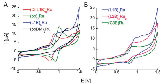
Fig. 3 Comparison between the cyclic voltammograms of (A) 0.5 mM intermolecular Ru complexes and (B) 0.5 mM ( L1B ) 3 Ru and 0.25 mM ( L2B ) 3 Ru 2 that were recorded in acetonitrile at rt. using a glassy carbon working electrode, platinum counter electrode, and Ag/AgNO 3 reference electrode. Scan rate: 100 mV s -1 .
