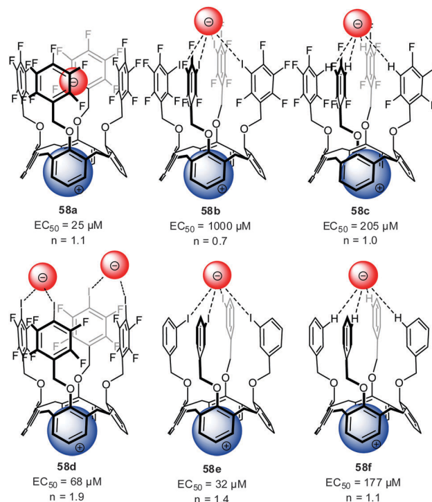
Fig. 32 Molecular structure of the investigated ion pair receptors 58 for transport studies by Mentrangolo, Resnati and Matile et al. 10a
