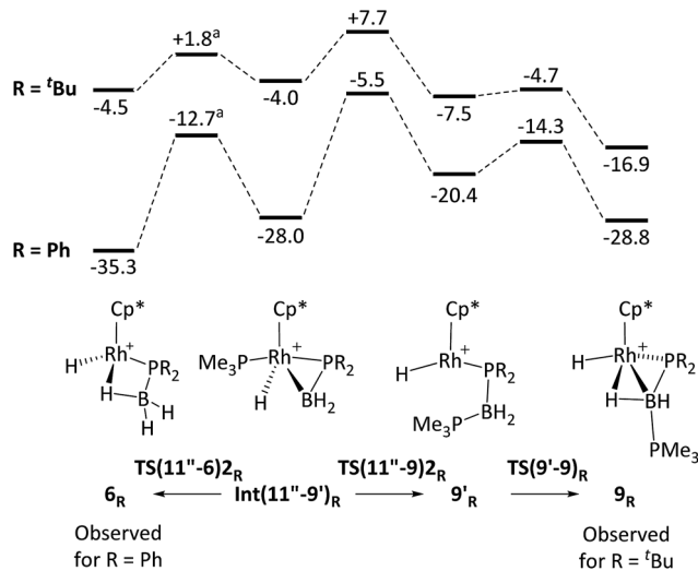
Fig. 7 Computed free energy reaction profiles ( \text{kcal mol}^{-1} , BP86-D3 (DCM) level) for formation of 6_R and 9_R from phosphino-borane adducts \text{Int}(11''-9')_R : ( R = {}^t\text{Bu} and \text{Ph} ). All free energies are quoted relative to 10 set to 0.0 \text{ kcal mol}^{-1} . a An intermediate corresponding to a ca. 90^\circ rotation of the phosphino-borane ligand was located between \text{Int}(11''-9')_R and 6_R and only the energy of the higher-lying transition state is indicated. See text and ESI† for full details.
