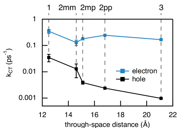
Fig. 7 Experimental charge transfer rate constants for electron (blue) and hole (black) transfer vs. the donor–acceptor distance. The donor–acceptor distance is only used for the purpose of visualization. The error bars are determined from multiple measurements.
