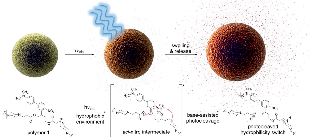
Fig. 1 Visible light irradiation of particles composed of polymer 1 in aqueous media induces swelling and release of molecular cargo. Tertiary amines within the polymer backbone assist deprotonation of the aci -nitro intermediate in the hydrophobic particle microenvironment, leading to \beta -elimination and photocleavage in favour of photorearrangement.
