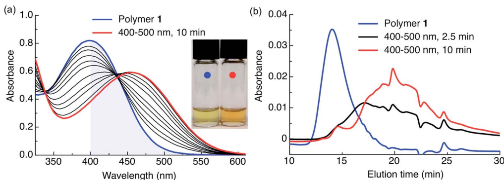
Fig. 3 Polymer 1 photodegrades upon irradiation with visible light in hydrophobic environments. (a) Spectral changes in the UV-Vis spectrum of polymer 1 irradiated in \text{CH}_2\text{Cl}_2 ( 0.04\text{ mg mL}^{-1} , 0.5\text{ mL} ) with visible light ( \lambda_{\text{ex}} = 400\text{--}500\text{ nm} , 0.18\text{ W} , 0.21\text{ W cm}^{-2} ). The blue shaded area highlights visible light absorption. Inset: color change following complete photoconversion. (b) GPC chromatogram of polymer 1 before (blue trace, M_w = 31.7\text{ kDa} , \text{PDI} = 2.7 , PMMA standard) and after irradiation in \text{CH}_2\text{Cl}_2 ( 0.04\text{ mg mL}^{-1} , 0.5\text{ mL} ) with visible light ( \lambda_{\text{ex}} = 400\text{--}500\text{ nm} , 0.18\text{ W} , 0.21\text{ W cm}^{-2} ) for 2.5 min (black trace) and 10 min (red trace). Absorbance sampled at 300\text{ nm} ; peak at 24\text{ min} is the toluene internal standard.
