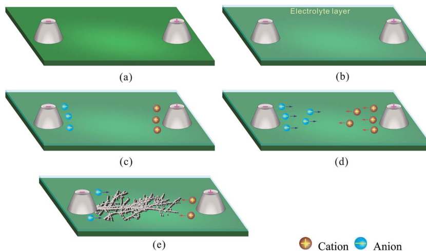
Fig. 3 The schematic diagrams of Sn solder alloy joints (a) ECM sample, and ECM process: (b) electrolyte layer formation, (c) dissolution of metal, (d) ion transport and (e) deposition of metal ions (dendrites growth).
