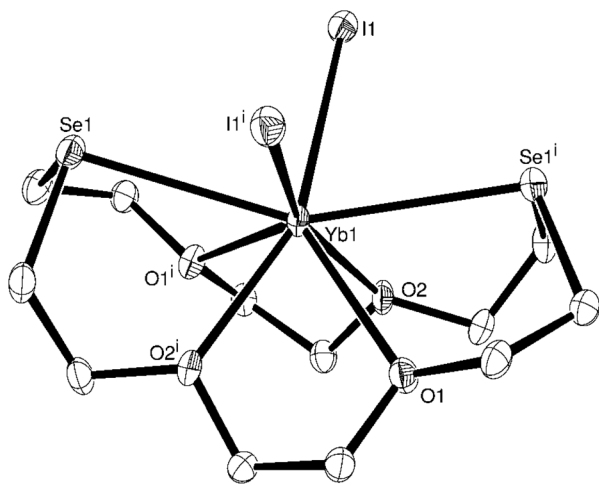
Fig. 1 View of the structure of [\text{YbI}_2(\text{18})\text{aneO}_4\text{Se}_2] showing the atom labelling scheme. The displacement ellipsoids are drawn at the 50% probability level and H atoms are omitted for clarity. Symmetry operation: i = -x, y, 1/2 - z . Selected bond lengths (Å) and angles ( ^\circ ): \text{Yb1}-\text{I1} = 3.1699(5) , \text{Yb1}-\text{Se1} = 3.1036(7) , \text{Yb1}-\text{O1} = 2.624(3) , \text{Yb1}-\text{O2} = 2.472(3) , \text{O1}-\text{Yb1}-\text{O1}^i = 117.98(14) , \text{O1}-\text{Yb1}-\text{O2} = 76.42(10) , \text{O1}^i-\text{Yb1}-\text{Se1} = 65.00(7) , \text{O2}^i-\text{Yb1}-\text{Se1} = 70.00(7) , \text{Se1}^i-\text{Yb1}-\text{Se1}^i = 152.86(2) , \text{I1}-\text{Yb1}-\text{I1}^i = 100.488(19) .
