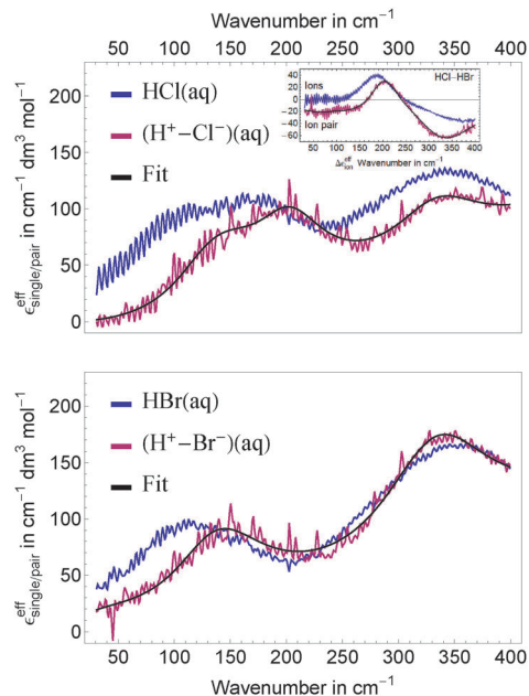
Fig. 6 Comparison of single ion and ion pair extinction spectra for HCl (top) and HBr (bottom). The inset in the top panel shows the extinction differences HCl–HBr for single ions (in blue) and ion pairs (in red).
