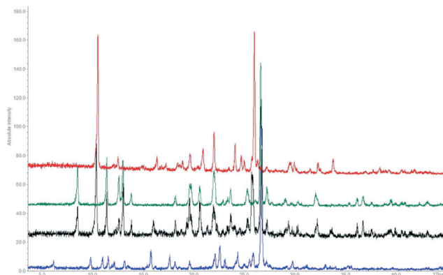
Fig. 14 PXRD pattern of SA-PTU-2MeCN (blue) compared with desolvated sample (black), sinapic acid (green), and 6-propyl-2-thiouracil (red).
