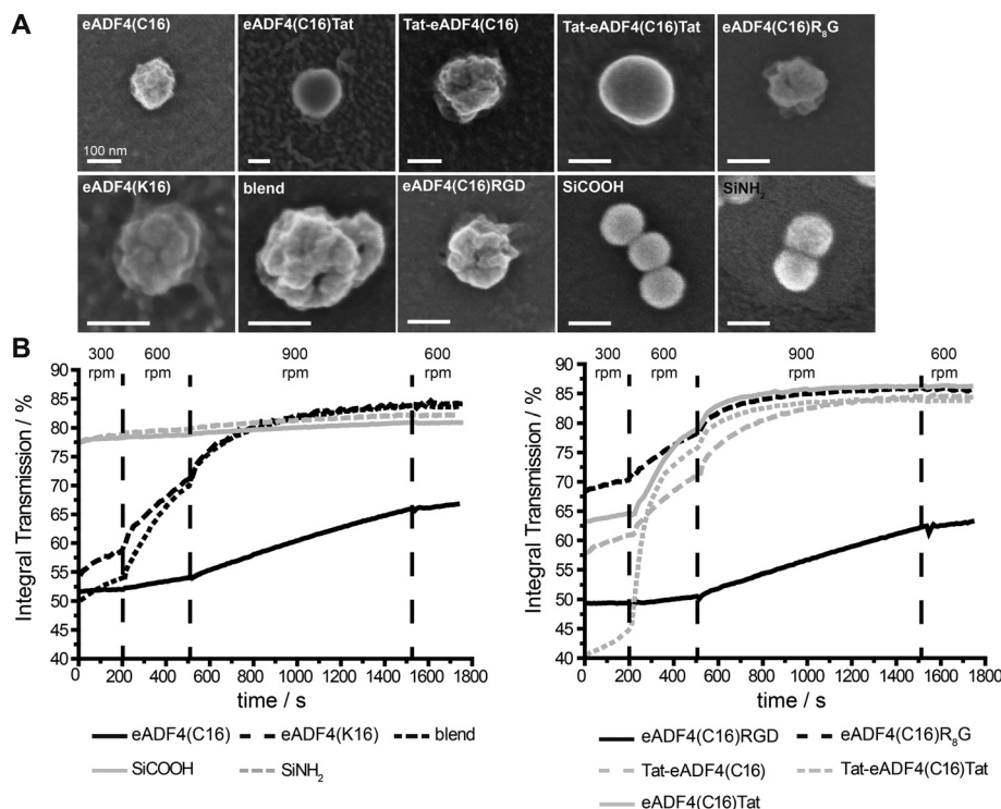
Fig. 2 SEM images (A) and colloidal stability analysis (B) of spider silk and control silica particles. For SEM, spider silk particles were prepared from a 0.1 \text{mg ml}^{-1} solution in EMiM[acetate] and analyzed in the dehydrated state. Colloidal stability of particles from a 2 \text{mg ml}^{-1} solution was determined in 10 mM KCl, pH 5.5. Scale bars: 100 nm.
