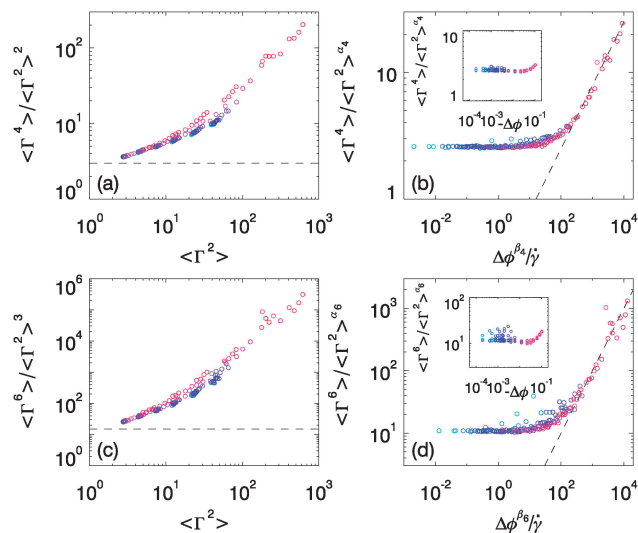
Fig. 5 Multiscaling relates \langle \Gamma^4 \rangle and \langle \Gamma^6 \rangle to \langle \Gamma^2 \rangle . (a) If the energy dissipation rate ( \Gamma^2 ) was normally distributed, \langle \Gamma^4 \rangle / \langle \Gamma^2 \rangle^2 = 3 (dashed line), and we see significant deviations of Gaussianity for large fluctuations ( \Gamma^2 ). (b) Scaling collapse for \langle \Gamma^4 \rangle / \langle \Gamma^2 \rangle^{\alpha_4} as function of \Delta\phi^{\beta_4} / \dot{\gamma} , for \alpha_4 = 2.33 \pm 0.05 and \beta_4 = 1.3 \pm 0.1 . The dashed line has slope 1/2. Inset: Data for \Delta\phi < 0 . (c) If the energy dissipation rate ( \Gamma^2 ) was normally distributed, \langle \Gamma^6 \rangle = 15 \langle \Gamma^2 \rangle^3 (dashed line), and we see significant deviations of Gaussianity for large values of \langle \Gamma^2 \rangle . Inset: Data for \Delta\phi < 0 . (d) Scaling collapse for \langle \Gamma^6 \rangle / \langle \Gamma^2 \rangle^{\alpha_6} as function of \Delta\phi^{\beta_6} / \dot{\gamma} , for \alpha_6 = 3.85 \pm 0.1 and \beta_6 = 1.1 \pm 0.2 . The dashed line has slope 1. Inset: Data for \Delta\phi < 0 .
