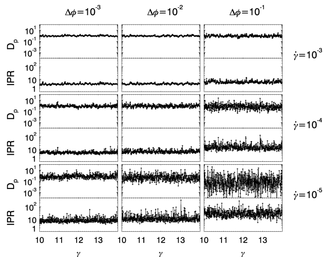
Fig. 3 The strain dependencies of the normalized energy dissipation D_p := \langle \Delta v^2 \rangle_x / \langle \Delta v^2 \rangle_{xt} and of the inverse participation ratio \text{IPR} := \langle \Delta v^4 \rangle_x / \langle \Delta v^2 \rangle_x^2 exhibit systematic trends with \Delta\phi and \dot{\gamma} .
