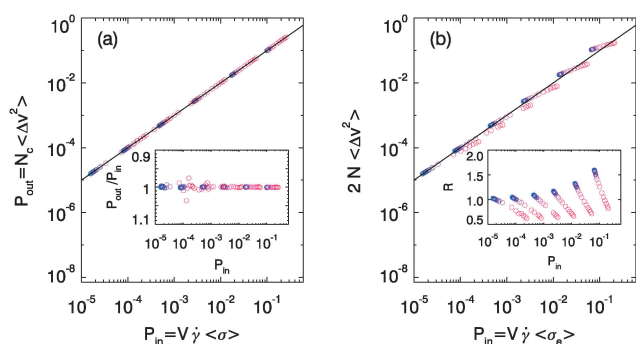
Fig. 1 (a) Scatter plot of P_{\text{in}} := V\dot{\gamma}\langle\sigma\rangle vs. P_{\text{out}} := N_c\langle\Delta v^2\rangle . Straight lines indicate equality, red (light) symbols denote high density and blue (dark) symbols denote low density. The inset shows that in our simulations P_{\text{in}} and P_{\text{out}} never differ more than a few percent. (b) The simplified version of the power balance equation, used in ref. 3, ignores the variation of the contact number and the contribution of the viscous stress. When we fix the contact number at four, we find that this simplified version works well for scaling, and that R := (2N\langle\Delta v^2\rangle)/(V\dot{\gamma}\langle\sigma_e\rangle) is within a factor two of unity.
