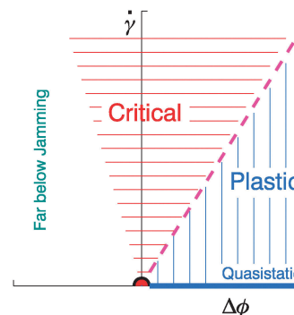
Fig. 6 Regimes in the (\Delta\phi, \dot{\gamma}) plane based on our scaling results for the moments of \Gamma . Our data indicates a crossover, at \dot{\gamma} \sim \Delta\phi^{\beta} for \beta \approx 1 (purple, dashed) which separates the critical and plastic regime as indicated. The quasistatic regime can smoothly be reached from the plastic regime. Our data clearly evidences critical behavior for \Delta\phi < 0 at finite flow rate, although the nature and location of the crossover to the deeply unjammed regime is unclear. Note that while the jamming point (red dot) plays a crucial role in organizing the physics, the line \Delta\phi = 0 has no particular significance for \dot{\gamma} > 0 .
