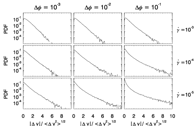
Fig. 2 The shape of the probability density function of the normalized velocity differences, |\Delta v|/\langle \Delta v^2 \rangle^{1/2} , varies strongly with packing fractions and strain rates as indicated. In this representation, a Gaussian appears parabolic and an exponential becomes a straight line.
