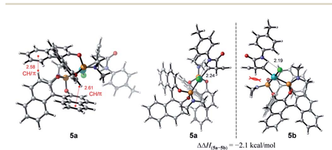
Fig. 4 Computed diastereomers 5a and 5b and their corresponding enthalpy difference ( \Delta\Delta H ) obtained at the SMD(THF)-M06-D3/def2-TZVP//TPSS-D3/def2-SVP/def2-TZVP for Cl and Pd level. Distances are in units of Å.
