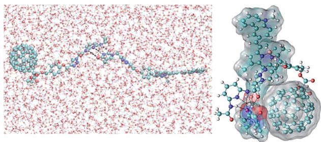
Fig. 9 Right: conformation of the B-3·C-1 complex in aqueous solution obtained from an MD simulation at 6.9 ns, showing the hydrogen bonds ( < 3 \text{ \AA} as indicated using black dotted lines) between B-3 and the C-1 motif. Left: the starting extended conformation used in the MD simulations. The white surfaces represent the solvent (water molecules) accessible surface areas of B-3 and the fullerene motif of the C-1 structure.
