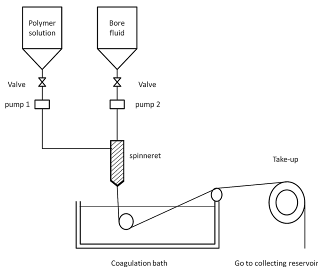
Fig. 20 Schematic diagram of the spinning apparatus for hollow fiber membrane.
