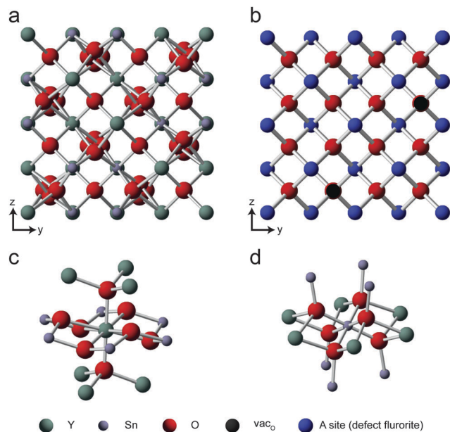
Fig. 1 Structure of (a) \text{Y}_2\text{Sn}_2\text{O}_7 pyrochlore and (b) a typical defect fluorite material. Green, small blue and red spheres denote Y ( i.e. , A site), Sn ( i.e. , B site) and O atoms, respectively. In (b), O vacancies are denoted by a black sphere, while the large blue sphere denotes the (single) cation site. Also shown are expansions of the nearest and next-nearest neighbour environments for the (c) eight-coordinated A site and (d) six-coordinated B site in the pyrochlore phase.
