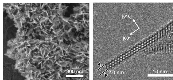
Fig. 4 SEM image of MFI nanosheets synthesized in a flake-like morphology (left), and TEM image of the cross-section of the flake (right). Adapted with permission from ref. 71. Copyright 2009 Macmillan Publishers Limited.
