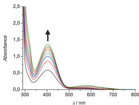
Fig. 1 UV/Vis spectra of a 500 μM solution of the complex [Cu(i) L hpz 1 (CH 3 CN) 2 ]PF 6 in CH 2 Cl 2 after addition of 50 eq. DTBP-H, 100 eq. NEt 3 and oxygenation between 15 min and 6 h; l = 1 \text{ mm} .
