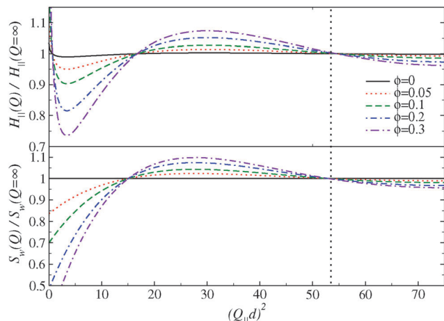
Fig. 6 The wall structure factor S_w(Q) and the hydrodynamic function H_{||}^s(Q) in a Q_{||} -scan at fixed Q_{\perp}d = 2.36 and \kappa d = 2.08 for a selection of volume fractions. Both functions are normalised by their self-values at Q \rightarrow \infty . At (Q_{||}d)^2 \approx 53 we find an isosteric point for both functions (marked by the dotted vertical line), suggesting that the self-diffusion coefficients may be determined from the data collected in the vicinity of this point. The statement also holds sway for other components of H .
