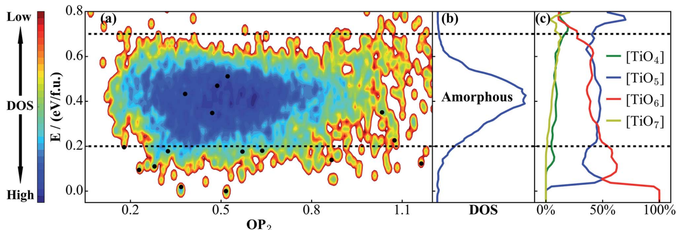
Fig. 5 (a) PES contour plot for \text{TiO}_2 distinct minima sampled from the SSW-NN global search. (b) Density of states (DOS) plot for \text{TiO}_2 phases in (a), showing that amorphous structures appear in the 0.2–0.7 eV f.u. ^{-1} window. (c) The percentage of differently coordinated Ti for \text{TiO}_2 structures. [\text{TiO}_5] and [\text{TiO}_6] are the main structural features for amorphous structures. Also see the Fig. 2 caption for the meaning of the black dots.
