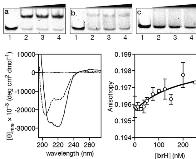
Figure 2 EMSA DNA binding studies results for the conjugate brH . (a) Lanes 1–4: [ brH ] = 0, 500, 700, 1000 nM, and 75 nM AP1 hs ·AT dsDNA. (b) Lanes 1–4: [ brH ] = 0, 500, 700, 1000 nM, and 75 nM of AP1 hs ·GC dsDNA. (c) Lanes 1–4: [ brH ] = 0, 500, 700, 1000 nM, and 75 nM of GC·AT dsDNA. Oligonucleotide sequences (only one strand shown): AP1 hs ·AT : 5'-CGCGTCATAATTGAGAGCGC-3'; AP1 hs ·GC : 5'-CGCGTCATCAGCGAGAGCGC-3'; and GC·AT : 5'-GACGGAATTTGAGAGCGTGC-3'. Bottom left: circular dichroism of a 5 \mu M solution (phosphate buffer pH 7.5) of brH (dashed line) and the same solution after the addition of 1 equiv. of the target AP1 hs ·AT dsDNA (solid lane). The contribution of the DNA to the CD spectrum has been subtracted for clarity. Bottom right: fluorescence anisotropy titration of a 25 nM solution of TMR- AP1 hs ·AT in the presence of increasing concentrations of brH . The best fit to a 1 : 1 binding model is also shown.
