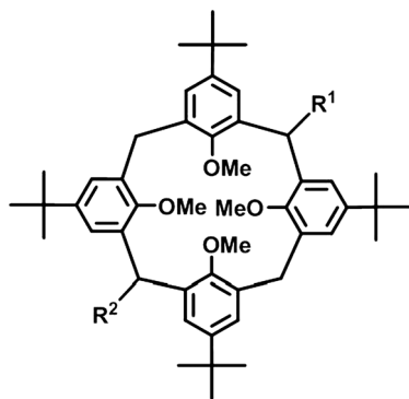
Scheme 1 Bridge non- ( R^1 = H , R^2 = H ), mono- ( R^2 = H ) and disubstituted calix[4]arenes. The lateral substituents act as spacers.
