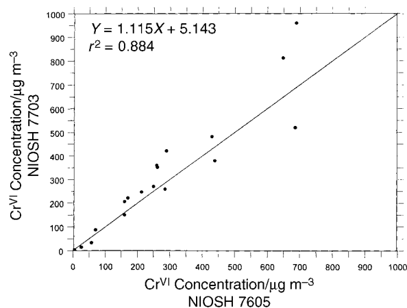
Fig. 3 Comparison of hexavalent chromium concentrations measured in field samples: NIOSH Method 7703 vs. NIOSH Method 7605. The line through the plot indicates unity slope and zero intercept, and does not represent the equation of the best fit line indicated on the figure.
